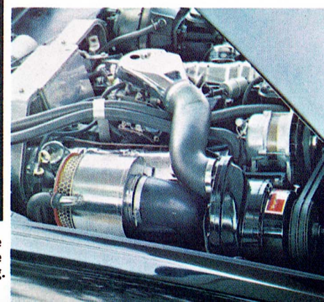
Paxton Supercharger. If you enjoy the thrill of exceptionally high performance, you get it with the optional Jet-Thrust V8 with Paxton supercharger. Gives you a 40 to 50% increase in reserve power as an extra margin of performance and safety for passing and highway cruising.
