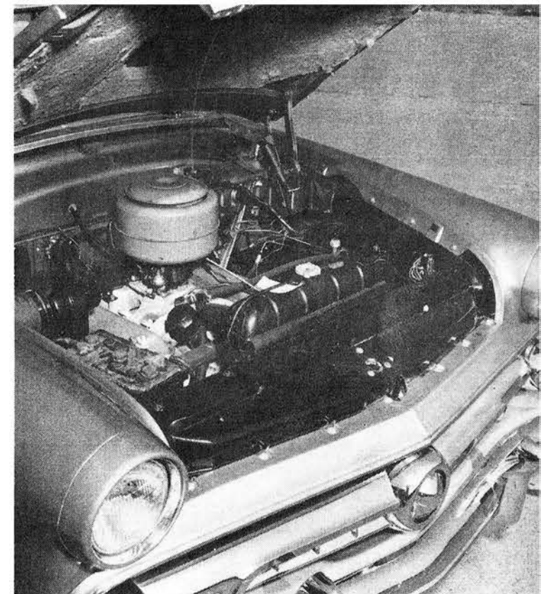
Switch in engines has had good and bad points from accessibility angle. However, the change in the suspension and frame clears oil pan area, permitting much easier removal
