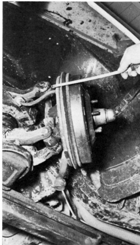
Front detail shows 1 3/16 inch anti-roll bar; heavy, short coil spring, and efficient center-plane brake.
