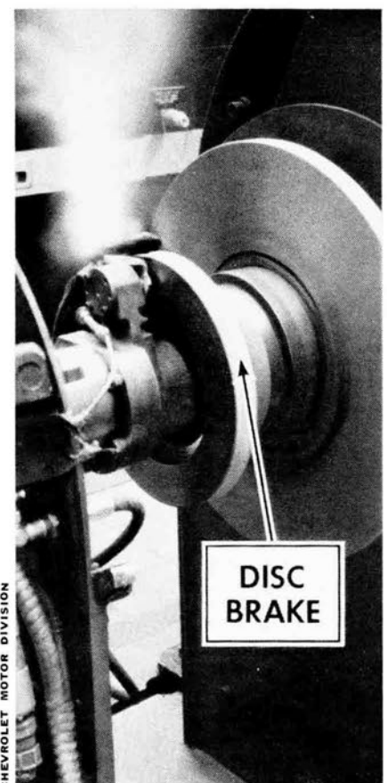
BRAKE DYNAMOMETER proved components. Discs attained temperature of 1200° F.
