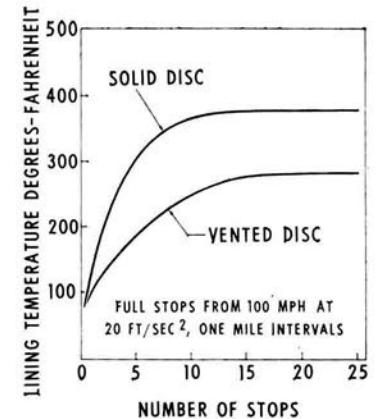
VENTED DISC gave significant reduction in lining temperatures during testing.
