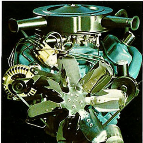
383-cu.-in. V8, 2-bbl. or 4-bbl., optional on Charger
