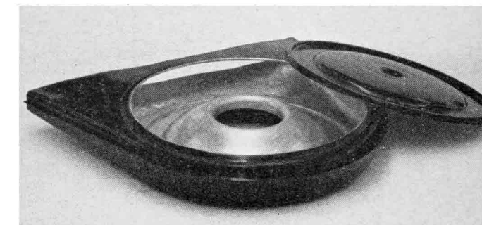
SPECIAL AIR intake chamber is designed for smooth, easy entry of ram air at 160-plus mph. SLIGHTLY exaggerated dotted lines show how cylinder bores are scalloped for better airflow with oversize valves.
