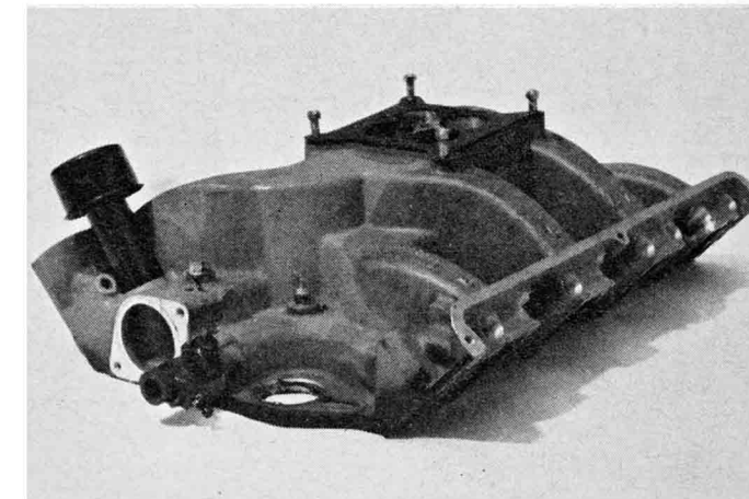
EXTRA HEIGHT of 1964 manifold is obvious; no spacer is required.
