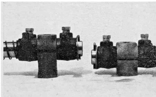
THE ROCKER shaft is not lower; the head is thicker and shorter brackets (right) provide a sturdier support.
