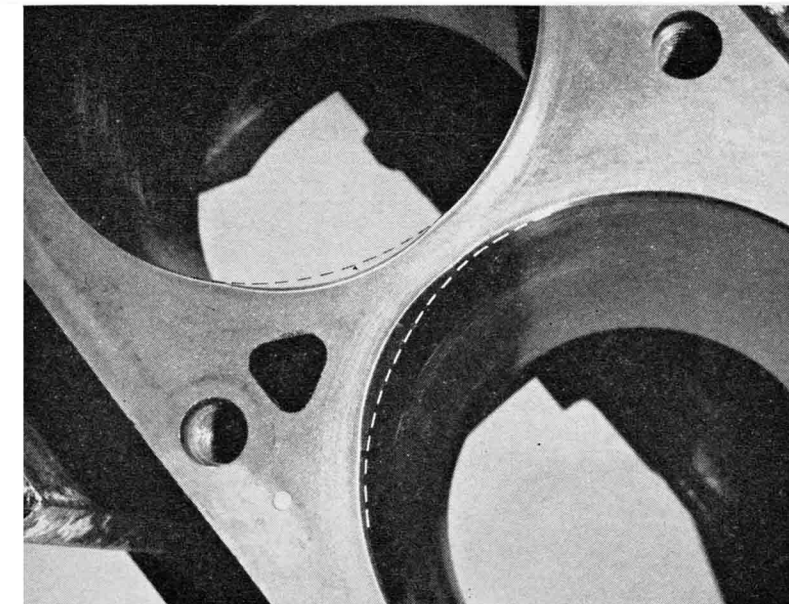
SPECIAL AIR intake chamber is designed for smooth, easy entry of ram air at 160-plus mph. SLIGHTLY exaggerated dotted lines show how cylinder bores are scalloped for better airflow with oversize valves.
