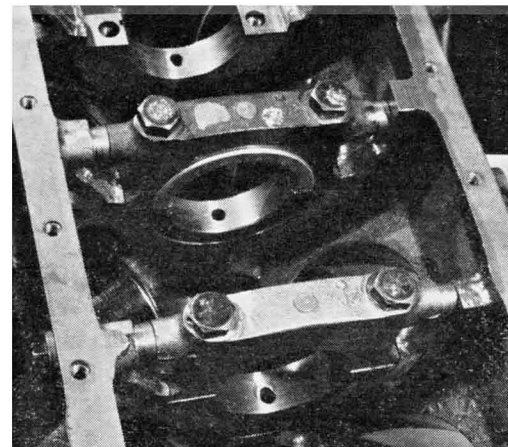
CROSS-BOLTED mains apply to center 3 bearings; the 6 bearings are well supported by the crankcase structure
