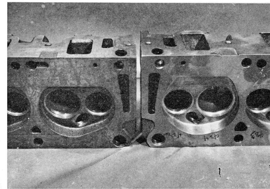
THE LATEST combustion chamber (right) is machined with special scallops to match the cylinder bore machining.
