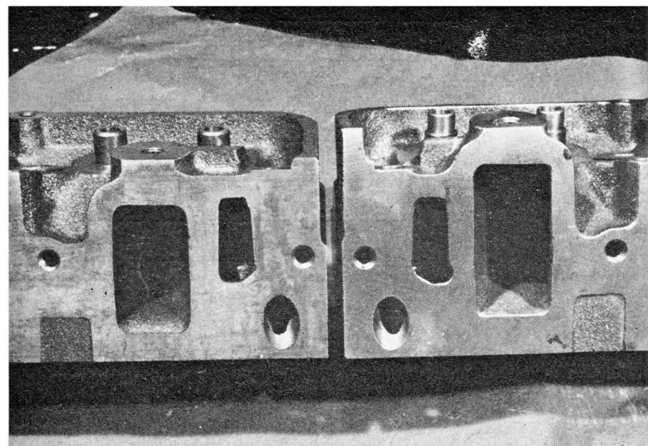
THE NEW intake ports (right) are raised and have more area for an easier turn with the high-rise manifold.
