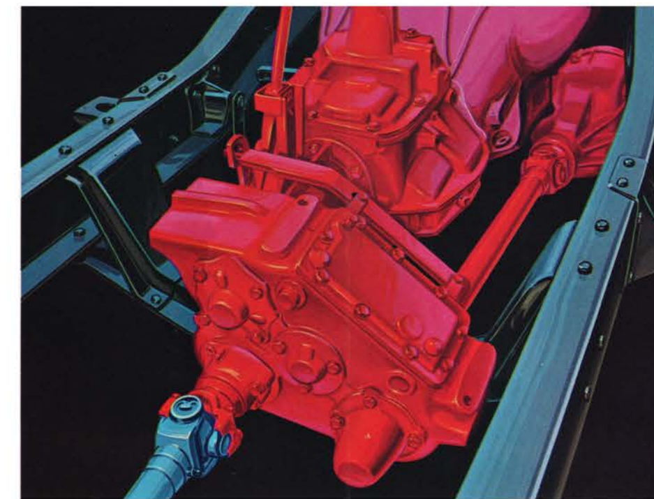
The 2-speed transfer case is bolted directly to the transmission. This eliminates the propeller shaft linkage usually found between the two gear boxes. As a direct result, the GMC cab and body are closer to the ground, making it easier to get in and out. One simple lever from the transfer case controls the engagement of front-wheel drive as well as the high and low ranges. Power take-off openings are provided for accessory drives to the front or rear.
