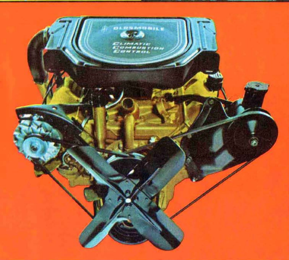
Jetfire Rocket V-8 with Oldsmobile's unique new Climatic Combustion Control.
