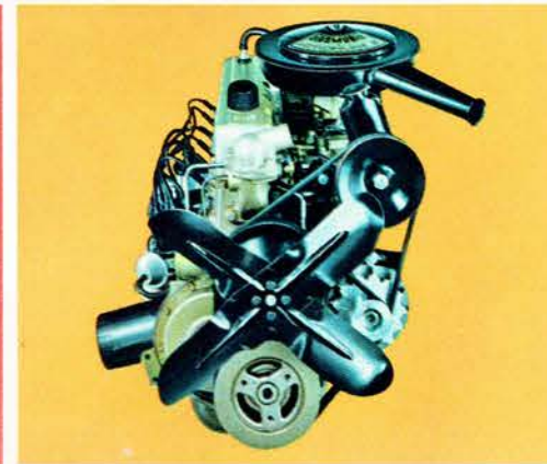
Action-Line 6. New in-line design delivers power efficiently, improves fuel economy, durability. 250-cu.-in. displacement. 155 hp. 240 lb.-ft. torque. 8.50-to-1 compression. Regular fuel. Available on F-85.
