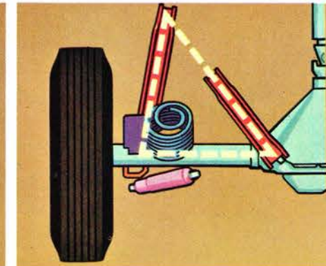
Twin-Triangle Rear Suspension incorporates four control arms, using triangular geometry, to greatly reduce rear-end squat. Wide pivot points and a lightweight axle also help to keep every Olds on the level.
