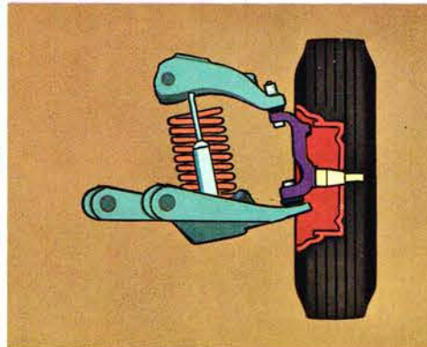
Pivot-Poise Front Suspension keeps Olds "steady as she goes!" "A" frame upper and lower control arms with wide pivot points combine with extra-wide wheel tread to improve stability regardless of road conditions.
