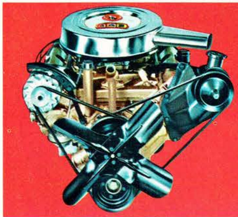
4-4-2 Rocket. Coolest new mill! New valve train, air cleaner, exhaust system. 400-cu.-in. 350 hp. 440 lb.-ft. torque. 10.5-to-1 compression. Quadrajt Carb. Premium fuel. Available on all 4-4-2 models only.
