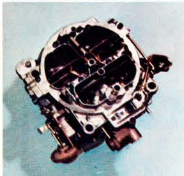
New Quadrajt Carb. 40% increase in capacity through air-metered secondary throttle bores. Primaries with smaller venturis for added economy.
