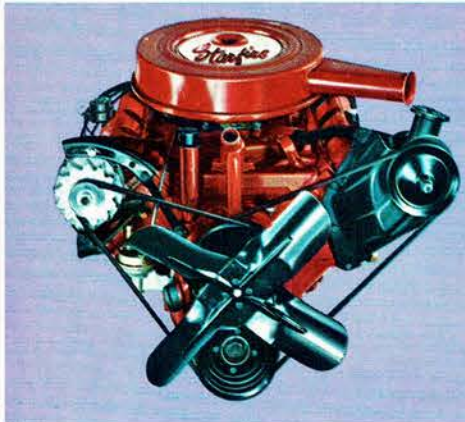
Starfire V-8. Quadrajt Carburetor. High-lift camshaft. 425-cu.-in. 375 hp. 470 lb.-ft. torque. 10.5-to-1 compression ratio. Premium fuel. Standard on Starfire. Optional on all Ninety-Eight and Delta 88 models.
