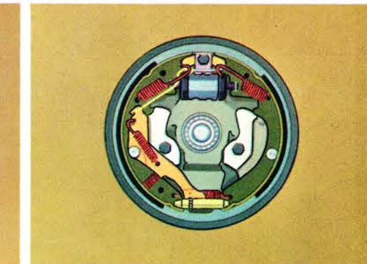
Air-Scoop Brakes have wide flange that sweeps up air to dissipate heat. Thick linings reduce wear. Large lining areas, plus organic compounds, aid stopping power. All brakes are self-adjusting, self-energizing.
