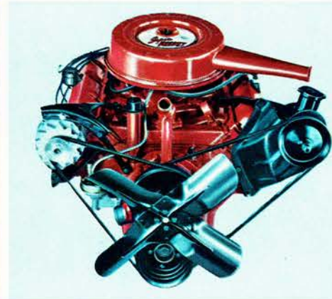
Super Rocket V-8. New 2-barrel carburetor. 310 hp. 450 lb.-ft. torque. 425-cu.-in. 10.25-to-1 compression. Premium fuel. Standard on Delta 88 and Dynamic 88. 300 hp regular fuel available, no extra cost.
