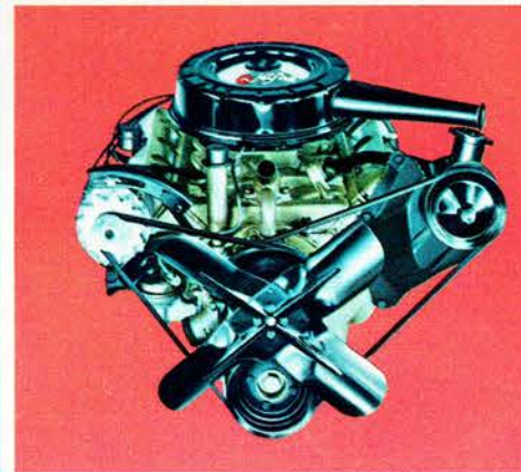
Jetfire Rocket V-8. Biggest V-8 in its class makes F-85 a top performer. 330-cu.-in. displacement. 250 hp. 335 lb.-ft. torque. 9.00-to-1 compression. Regular fuel. Available on F-85. Standard on Vista-Cruiser.
