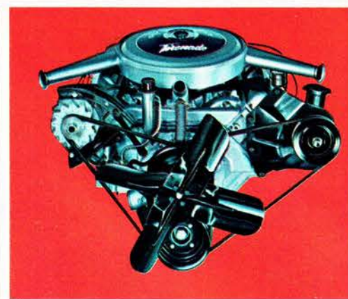
Toronado Rocket V-8. Oldsmobile's top-performing Rocket. Twin-snorkel air cleaner. Quadrajt Carb. 425-cu.-in. 385 hp. 475 lb.-ft. torque. 10.5-to-1 compression. Standard on both Toronado models.
