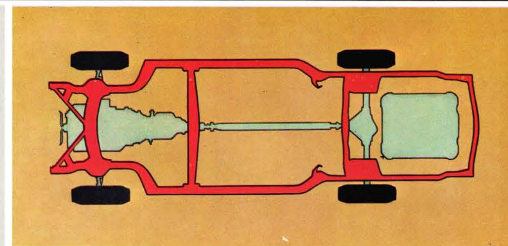
Guard-Beam Frame. Olds-pioneered perimeter-type design cradles and protects the chassis, improving passenger comfort and permitting greater ground clearance. Rigidity is increased, twisting forces minimized, thanks to rugged K-type braces at front wheels and swept-back torque boxes. It all adds up to a smooth, solid ride in every 1966 Rocket Action Oldsmobile.
