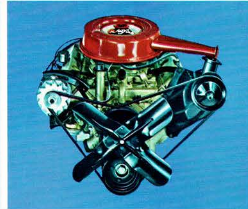
Jetfire Rocket V-8. 330-cu.-in. 260 hp. 355 lb.-ft. 10.25-to-1. Premium fuel. Standard on Jetstar 88. Regular fuel, 250-hp version available at no extra cost. Quadrajt, 320-horsepower version optional at extra cost.
