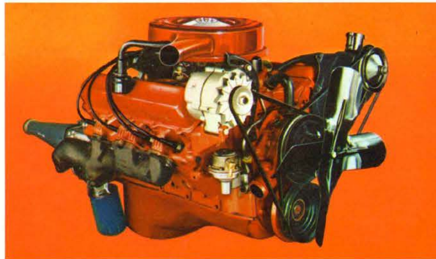
Oldsmobile's newest Rocket—the 425-cubic-inch, 310-h.p. Super Rocket V-8—is standard on Dynamic 88. 360-h.p. Super Rocket, or 370-h.p. Starfire on Delta, optional at extra cost. Regular-gas 300-h.p. version is optional at no extra cost.
