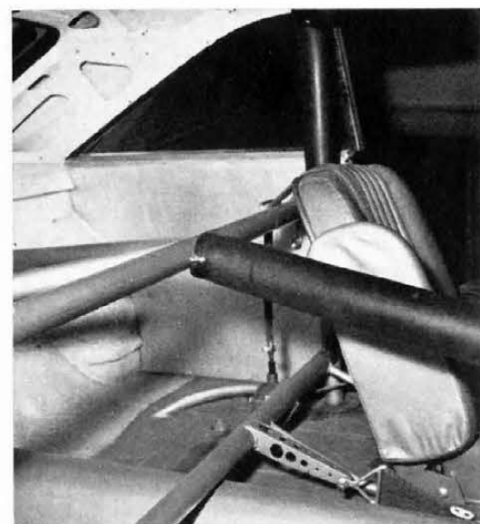
ROLL CAGE inside cockpit is constructed of 1.75 in. Shelby tubing; rubber wrapping protects driver. Below: tabs for door-bolts are welded in place.
