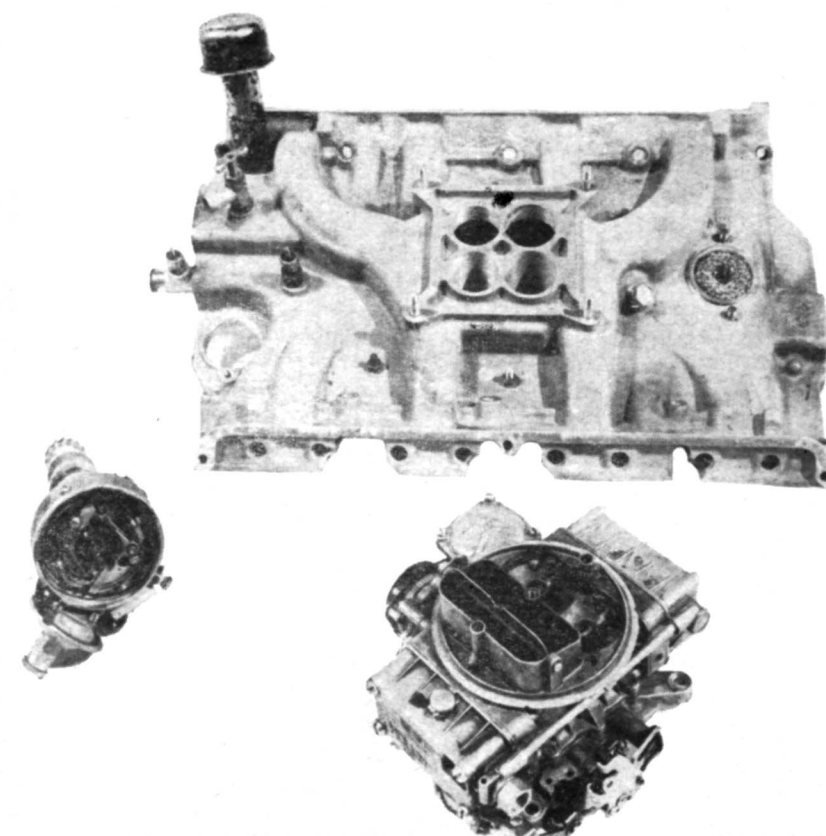
ALUMINUM INTAKE MANIFOLD (top) is responsible for reducing engine weight by some 40 lbs. Ignition (left) reportedly has no vacuum advance and is equipped with dual points. Holley four-barrel handles carburetion chores on the 360-hp engine.
