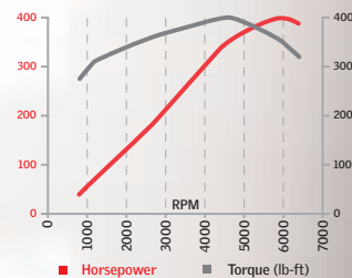
SQUARE DEAL: TORQUE IS THE FORCE THAT DELIVERS ACCELERATION; HORSEPOWER ALLOWS A VEHICLE TO SUSTAIN SPEED. THE LS2 V8 COUPLES 400 HORSEPOWER WITH 400 LB-FT OF TORQUE. IT'S NOT JUST THAT THE FIGURES ARE HIGH, BUT THAT THEY'RE IN AN IDEAL BALANCE FOR PERFORMANCE. STEP ON THE GAS, AT ANY RPM, AND YOU GET RESULTS.
